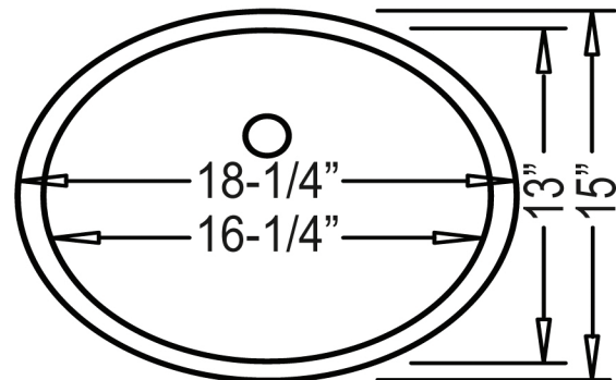
Product Diagram
